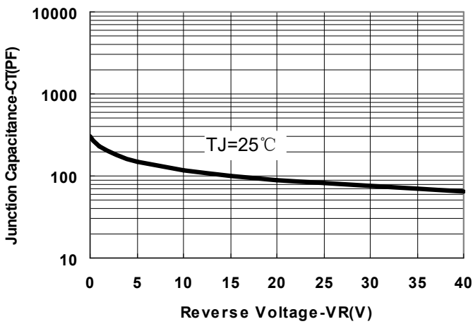
Fig.1-Typical Junction Capacitance
